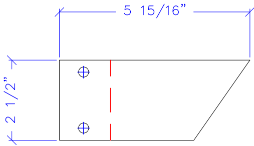
PLATE DETAIL
