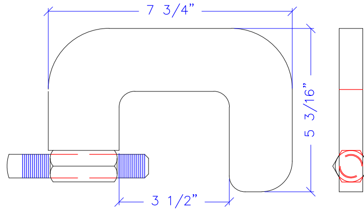
3 1/2" OPENING C-CLAMP
