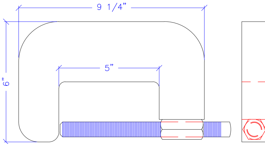
SPECIAL HD C-CLAMP
