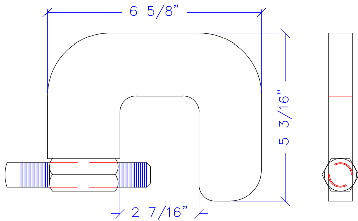
STANDARD HD C-CLAMP
