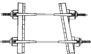
She-Bolts
