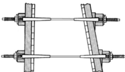
She-Bolts
